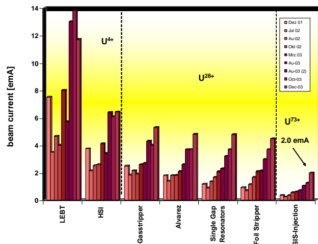
Fig. 2: Improvement of the UNILAC-Uranium beam intensities [2].
