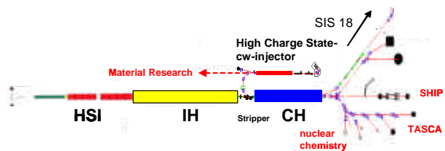
Fig. 4: Conceptual layout of a multipurpose high intensity heavy ion facility.
