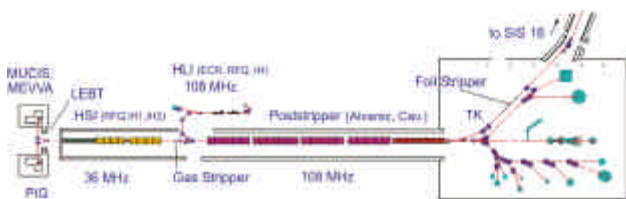
Fig. 1: Schematic overview of the GSI UNILAC and experimental area.
